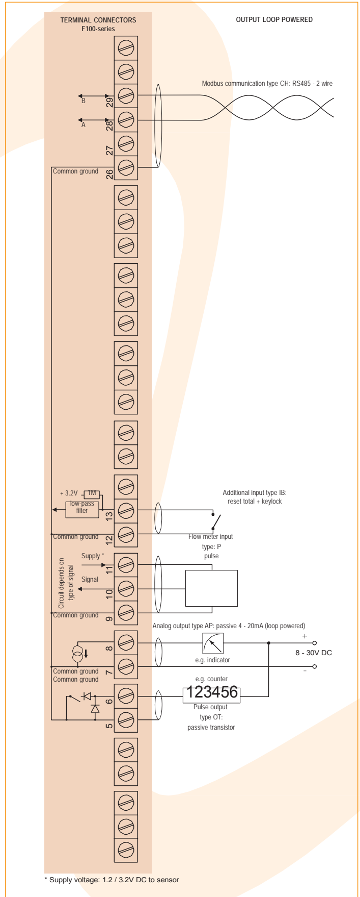
Typical wiring diagram F110-P-AP-CH-IB-OT-PX
