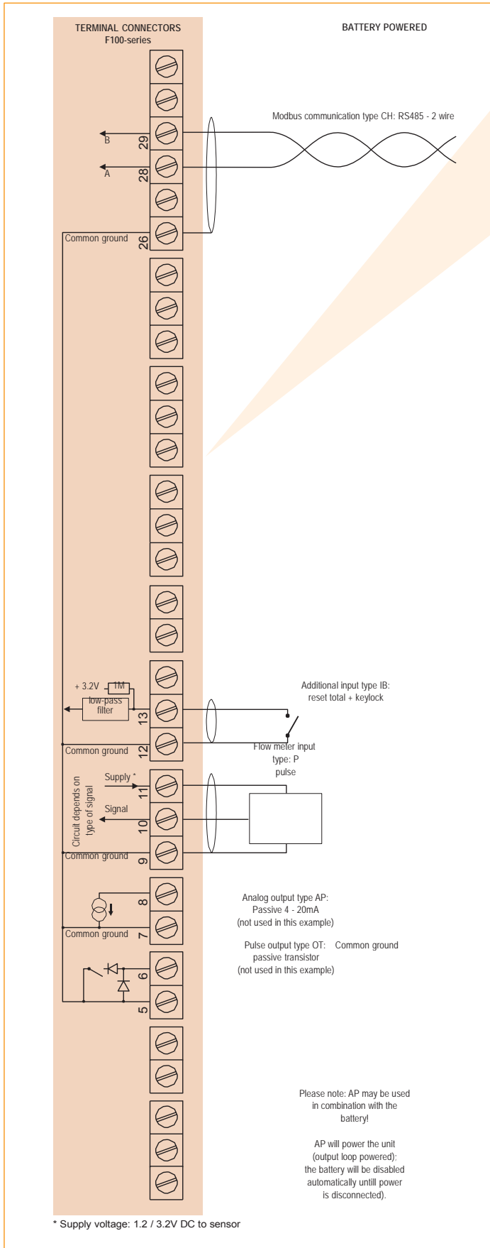
Typical wiring diagram F110-P-(AP)-CH-IB-OT-PB
